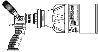
FIG 4 - FJ-MX-D Shown on Twister Nozzle
