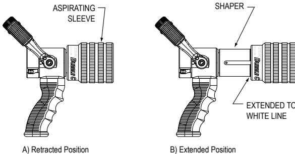
FIGURE 3 BUBBLE CUP OPERATING POSITIONS
