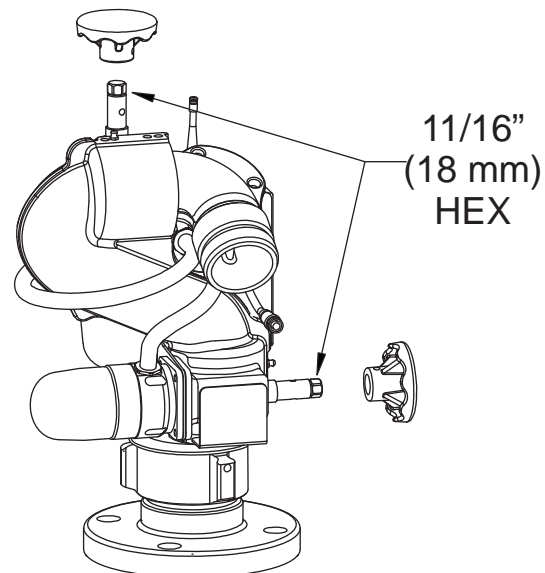
Fig 5.1 Wrenching Hexes on Drive Shafts
