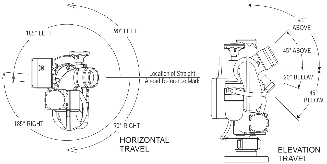
Fig 4.2B Travel Ranges Relative to Straight Ahead Reference Mark
