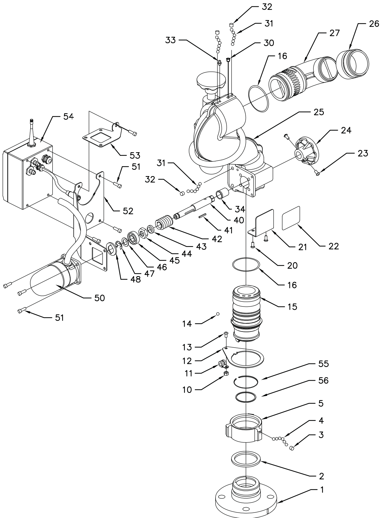
Fig 9.2 Tornado RC Exploded View
