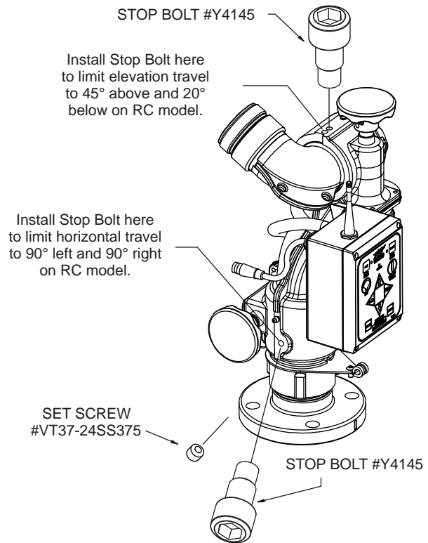
Fig 4.2C Stop Bolt Use
