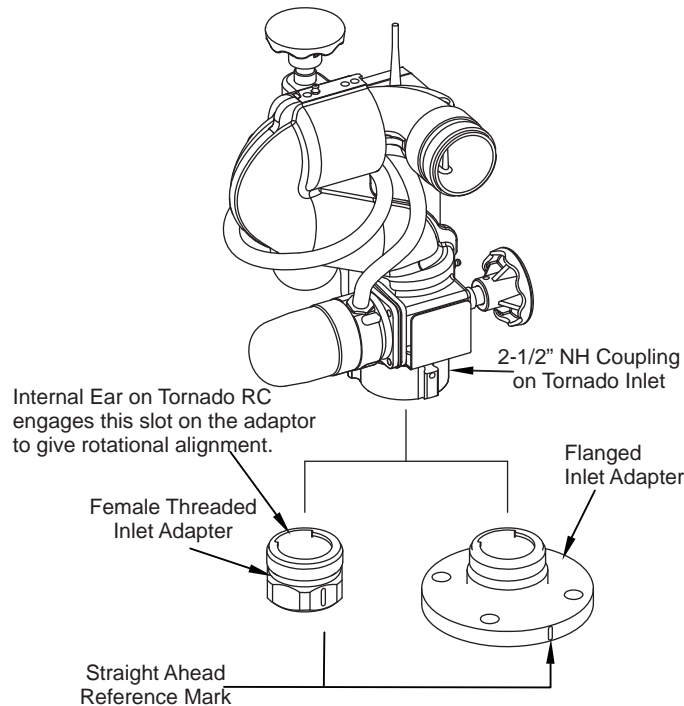
Fig 4.2A Inlet Adapter and Straight Ahead Reference Mark
