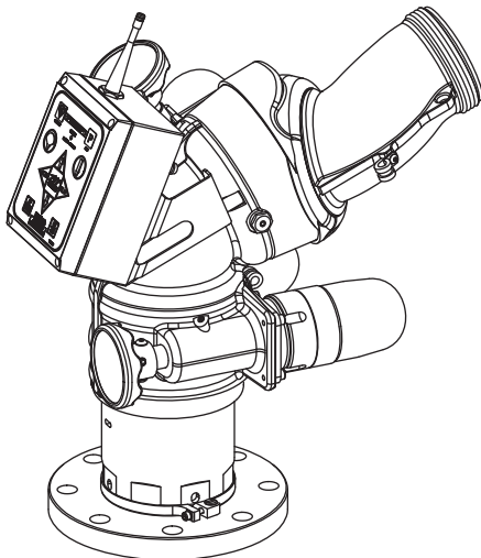
Figure 3.2D Electric Monsoon RC for Ladders or Platforms
