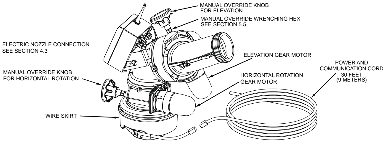
Figure 3.2C Electric Monsoon RC Monitor
