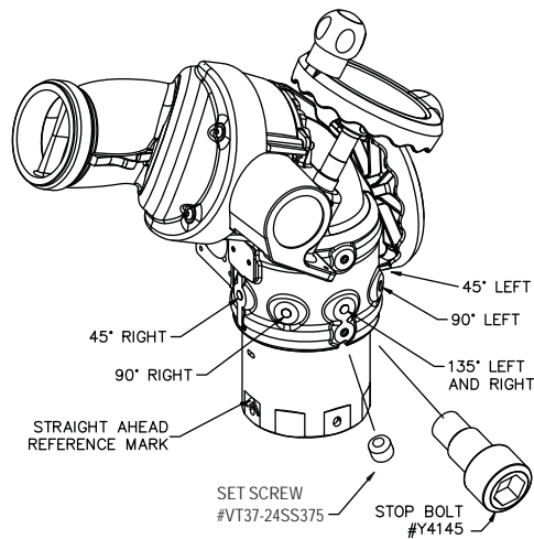
Fig 4.2.2A Horizontal Rotation Travel Limits
