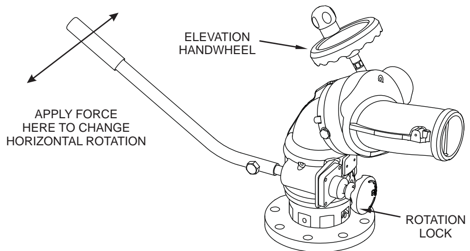
Figure 5.3 Tiller Bar Model Controls
