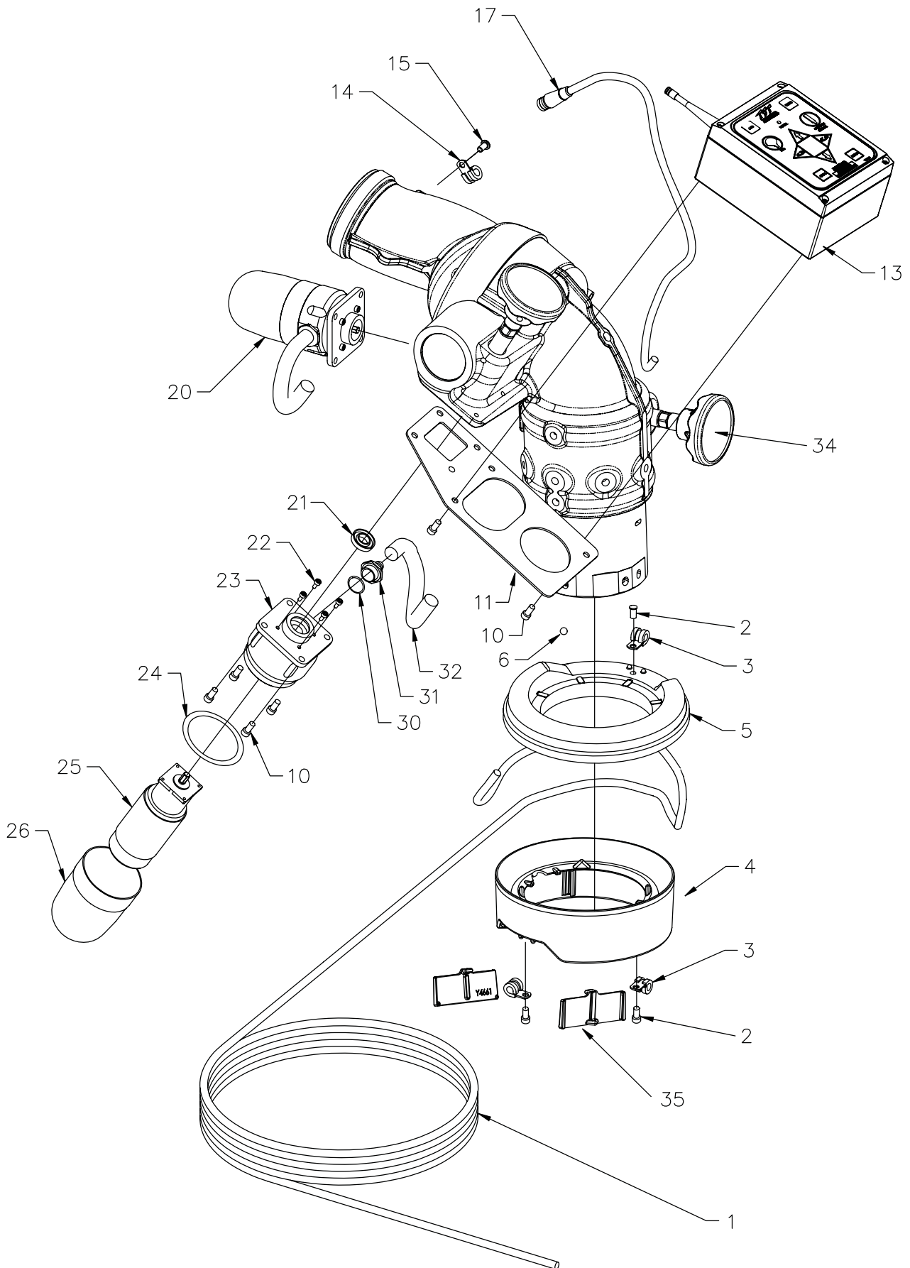
Fig 9.2 Monsoon RC Exploded View of Electrical Parts
