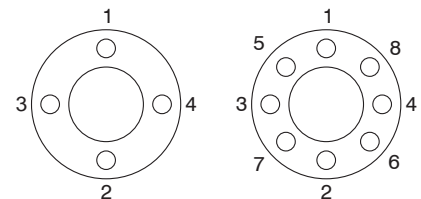
Fig 4.1 Flange Bolt Tightening Sequence
