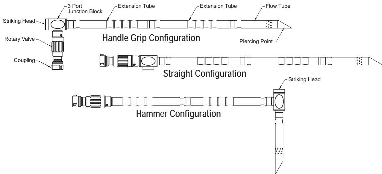
Figure 2.0 Part Identification
