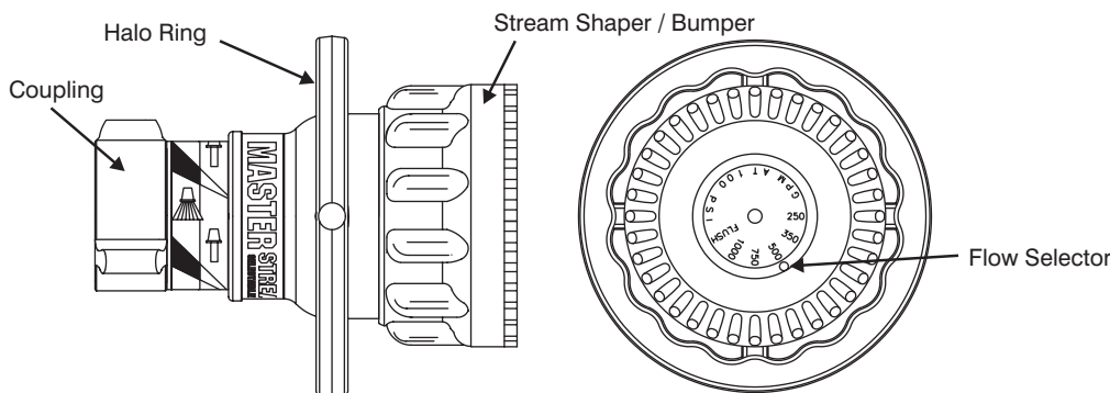
FIG 1B - Masterstream 1000 Selectable Gallonage Nozzle
