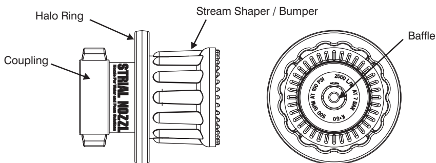
FIG 1A - Industrial Nozzle
