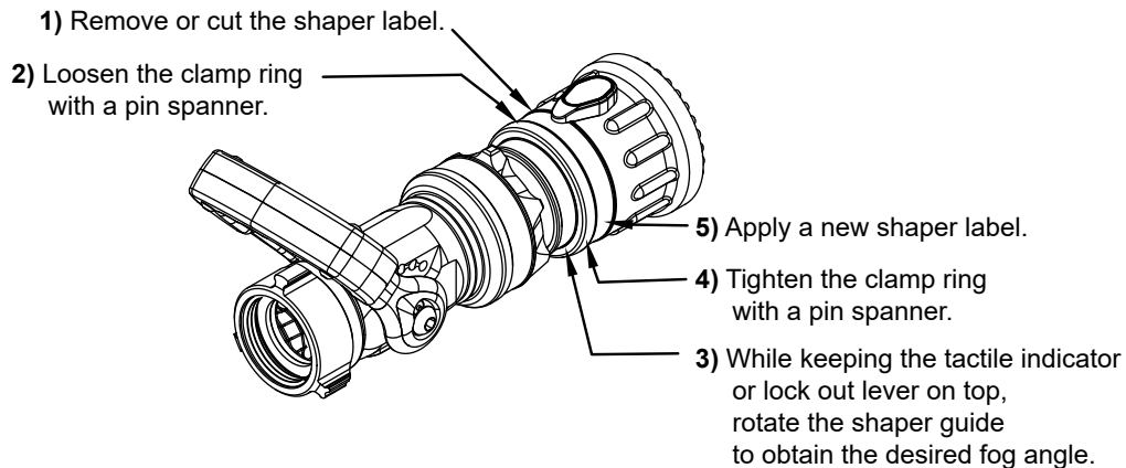
Figure 5.2.3 Fog Angle Adjustment
