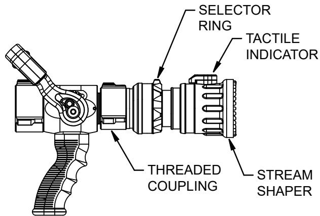
TIP ONLY NOZZLE (Shown With H-VOI Ball Valve)
