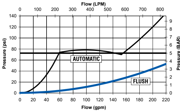
Figure 4.3B 1.5" G-Force 75 psi Automatics
