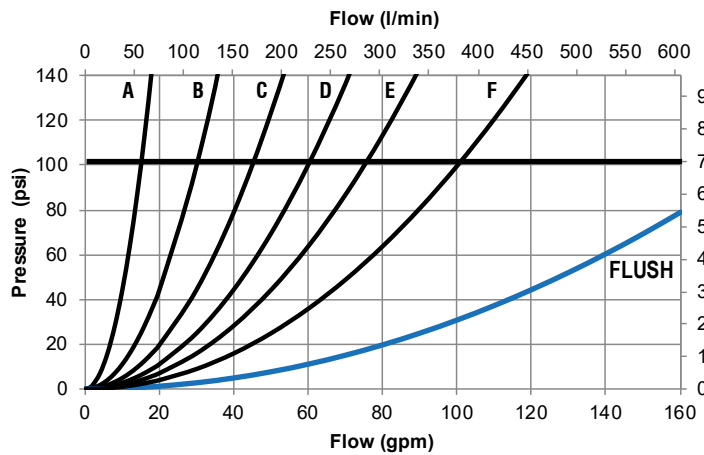
Figure 4.2C 1.5" G-Force 100 psi Fixed and Selectable Nozzles
