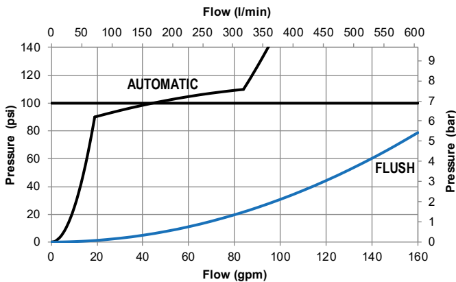
Figure 4.3C 1.0" G-Force 100 psi Automatic
