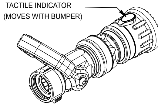
Figure 5.2.2 Shaper Tactile Indicator
