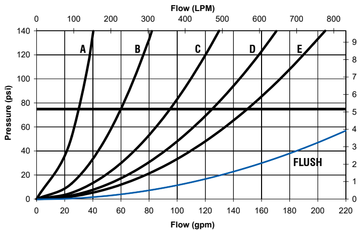
Figure 4.2B 1.5" G-Force 75 psi Fixed and Selectable Nozzles
