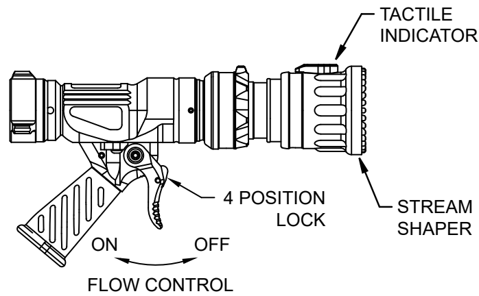
NOZZLE WITH IMPULSE TRIGGER VALVE SYSTEM
