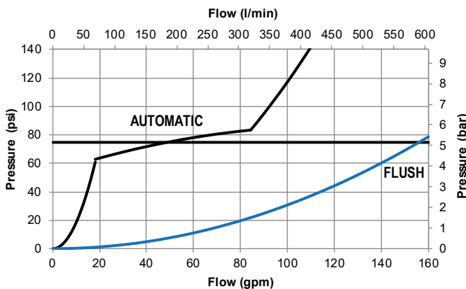
Figure 4.3D 1.0" G-Force 75 psi Automatic
