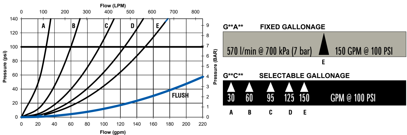
Figure 4.2A 1.5" G-Force 100 psi Fixed and Selectable Nozzles
