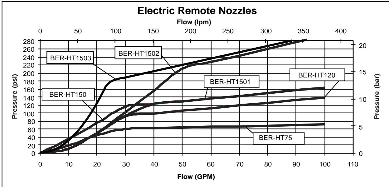
FIGURE 3.0 - FLOW CURVES
