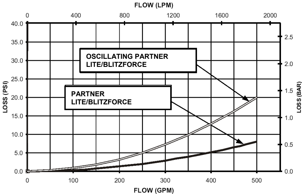
Figure C.1- Pressure loss chart
