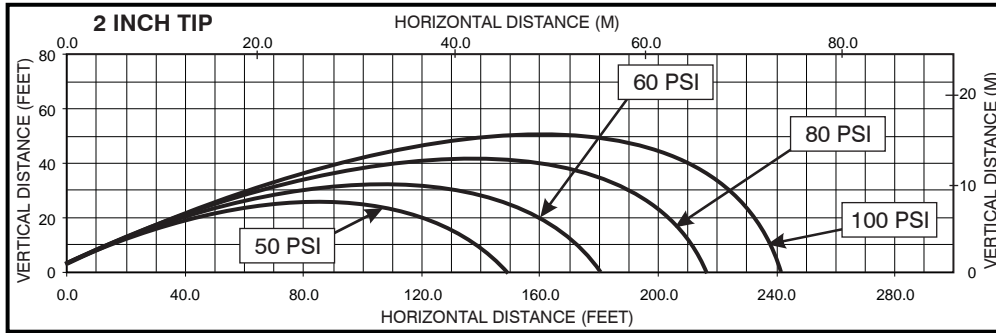
Fig 6.1C Stacked Tip Flow Graph
