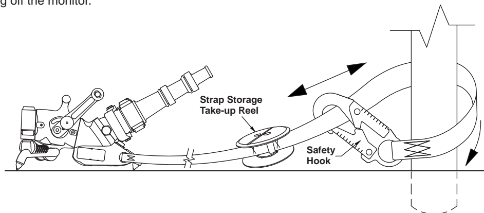
Figure 5.4 Tying Off of Blitz Lite Portable Monitor
