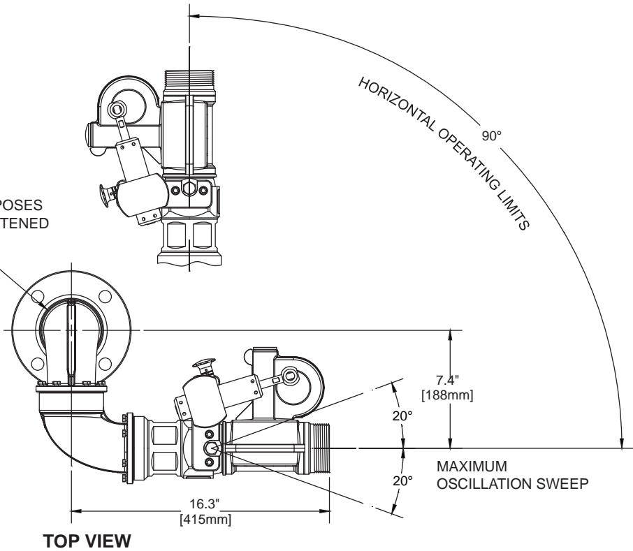
TOP VIEW
