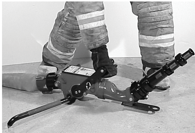
Figure 4.2 Advancing the Blitzfire with a Charged Hose
