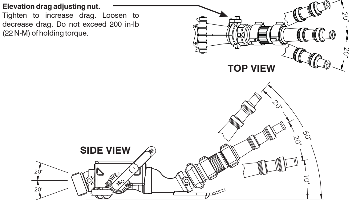
Figure 2.5 Inlet and Outlet pivots Range of Motion
