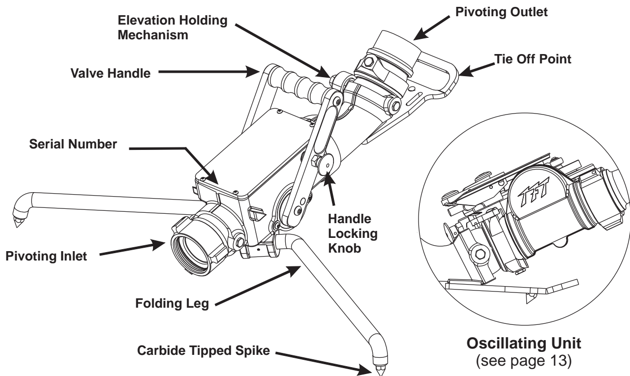
Figure 2.1 Blitzfire Parts and Controls
