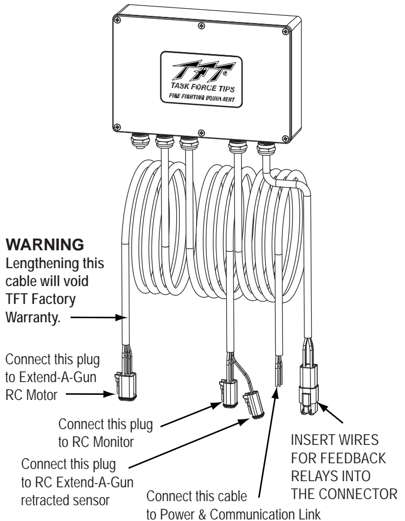
Figure 7.3 Control Box Wiring
