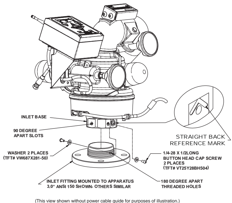
Fig 4.2.1A 3" Inlet Fitting Connection
